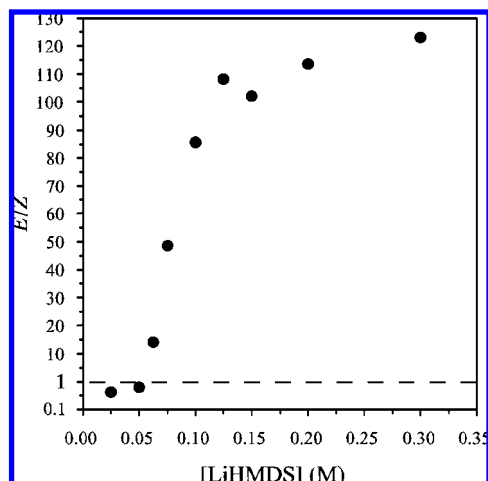
Figure 1. E/Z selectivity ( E -6: Z -6, eq 3) versus molarity (M) of LiHMDS in samples containing 0.10 M ketone 5 and 1.2 M excess Et 3 N in toluene at -78\text{ }^{\circ}\text{C} . 16
