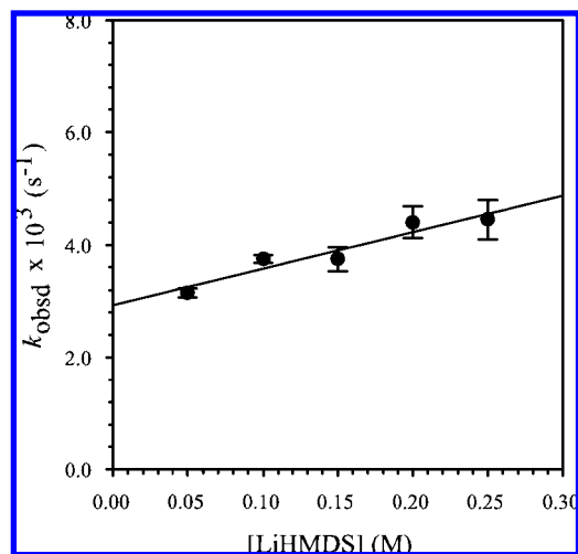
Figure 3. Plot of k_{\text{obsd}} versus [\text{LiHMDS}] in 4.0 M \text{Et}_3\text{N} /toluene solution for the enolization of 5-d 3 (0.005 M) by LiHMDS at -78\text{ }^\circ\text{C} . The curve depicts an unweighted least-squares fit to k_{\text{obsd}} = a[\text{LiHMDS}] + b , where a = 5 \pm 1 , b = 3.0 \pm 0.1 .
