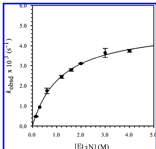
Figure 2. Plot of k_{\text{obsd}} versus [\text{Et}_3\text{N}] in toluene cosolvent for the enolization of 5-d 3 (0.005 M) by LiHMDS (0.10 M) at -78\text{ }^\circ\text{C} . The curve depicts an unweighted least-squares fit to k_{\text{obsd}} = a[\text{Et}_3\text{N}]/(1 + b[\text{Et}_3\text{N}]) , where a = 4.0 \pm 0.1 , b = 8.2 \pm 0.6 \times 10^{-1} .
